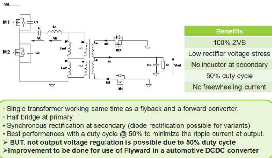
Figure 13: DC/DC converter topology
