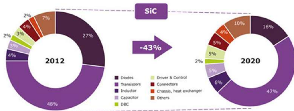
Figure 36: SiC- based inverter bill of material evolution from 2012 to 2020 with devices and components price erosion – source “SiC Modules, Devices and Substrates for Power Electronics Market”, Yole Développement, October 2014
